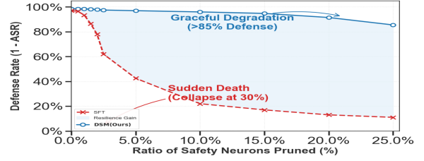
Figure 5: DSM demonstrates "Graceful Degradation," compared with SFT. The shaded area highlights the significant resilience gain provided by the mesh topology.
