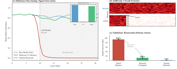
Figure 7: (a) Fine-tuning severs the safety circuit at localized neurons causing downstream dormancy. Grafting signal from the base model (Green) at source neurons restores defense. (b) Jailbreak attacks succeed by suppressing key safety neurons (bottom), causing cascaded failure. (c) Manually clamping these bypassed neurons to active states (Restored) drastically reduces Attack Success Rate.
