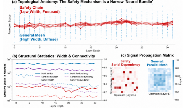
Figure 2: (a-b) Safety mechanisms appear as narrow and low-redundancy "neuron circuit" with minimal redundancy compared to both two the general circuits. (c) The downstream safety neurons' activation depends on a small number of upstream neurons, and they have the characteristic of a high causality.
