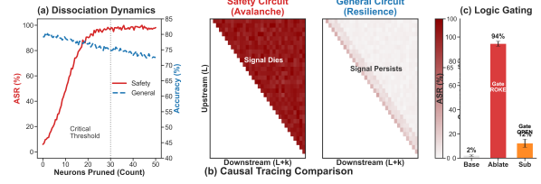
Figure 3: (a) Masking a minimal fraction ( < 0.8\% ) of safety neurons triggers immediate safety collapse (red), while general utility remains robust (blue). (b) Masking upstream layers ( L ) in the Safety Circuit triggers near-total downstream suppression (left). In contrast, the General Circuit (right) maintains signal flow via mesh-like structure. (c) Flow breaking results in high ASR, whereas residual subtraction maintains low ASR.
